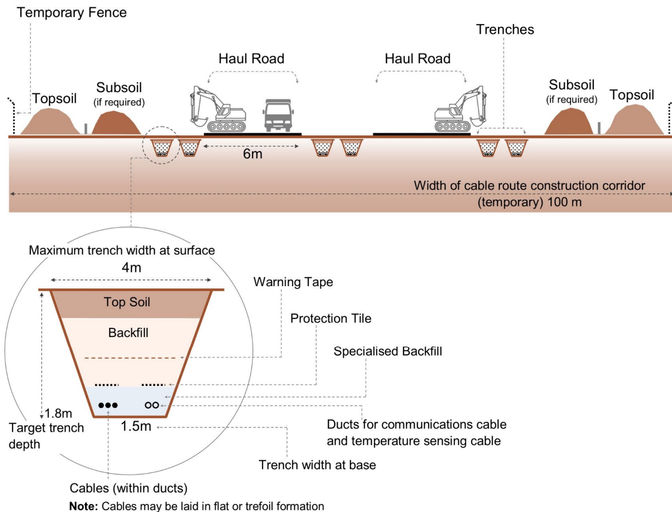
Diagram 3.1: Indicative temporary cable corridor cross section
