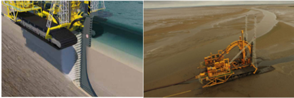
Plate 3.9: Example Cable Trenchers
